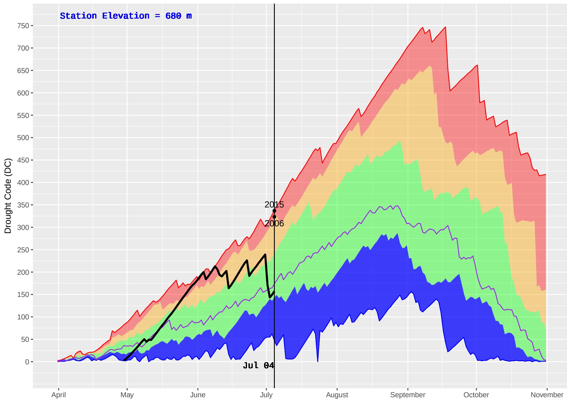
REVELSTOKE (363) : Historical (1995–2016) and Current (2018) Noon Drought Code (DC)
